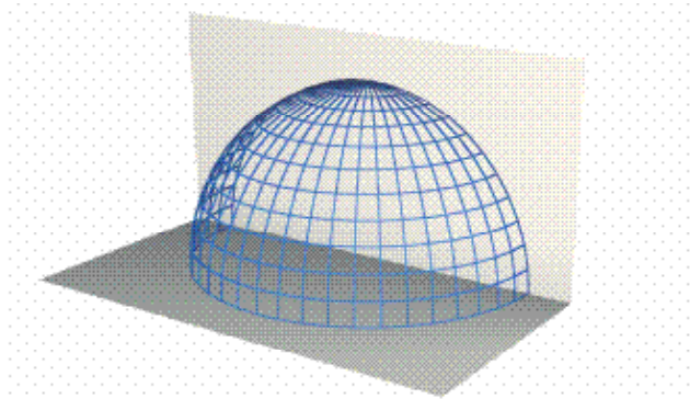
c Spherical radiation Q = 4
