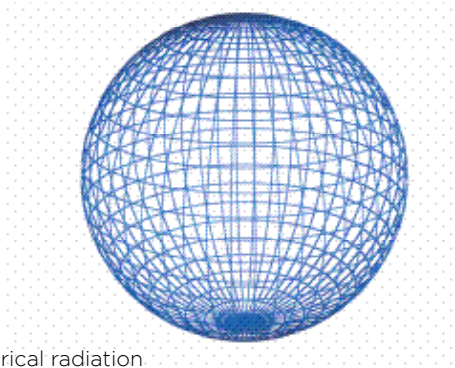
a Spherical radiation Q = 1
