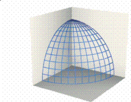
d Spherical radiation Q = 8
