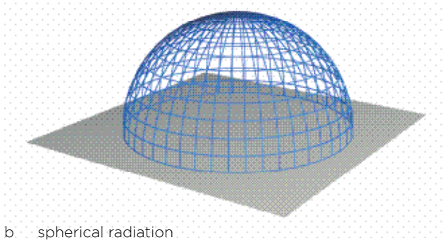
b Spherical radiation Q = 2
