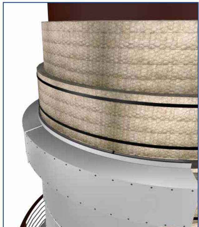
Figure 20. COLUMN DETAIL 2
