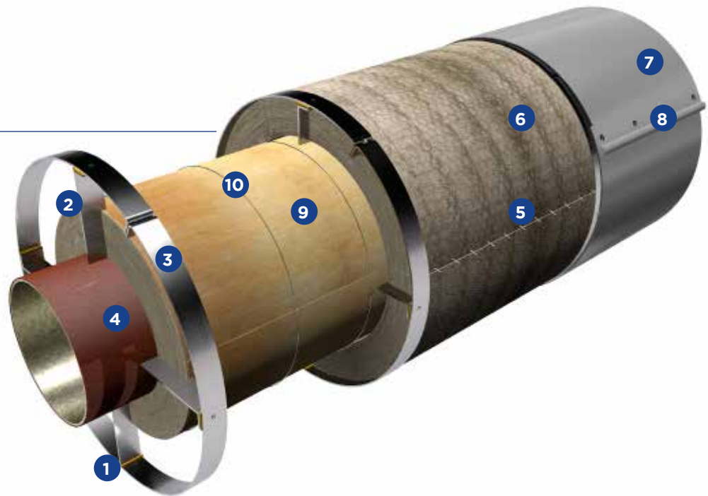
Figure 4. PIPING – Straight Pipe (Pipe Section + Wired Mat)
