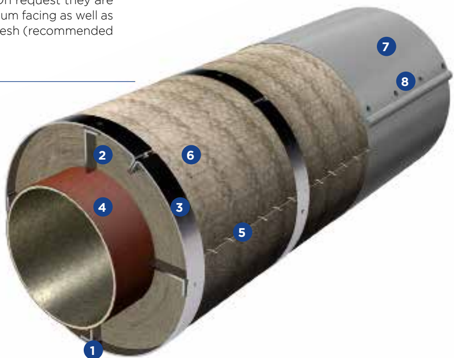
Figure 2. PIPING – Straight Pipe (Wired Mat)
