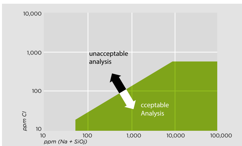
Acceptable analysis of water-leachable ions in mineral wool according to Karnes diagram
