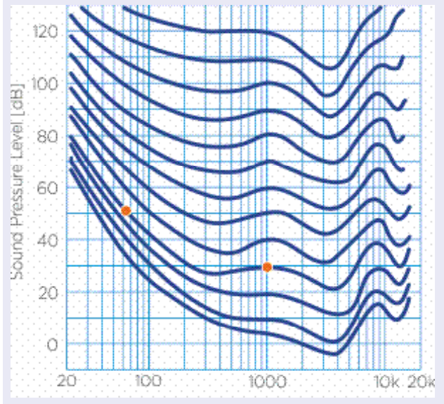
Fletcher-Munson equal loudness curve
