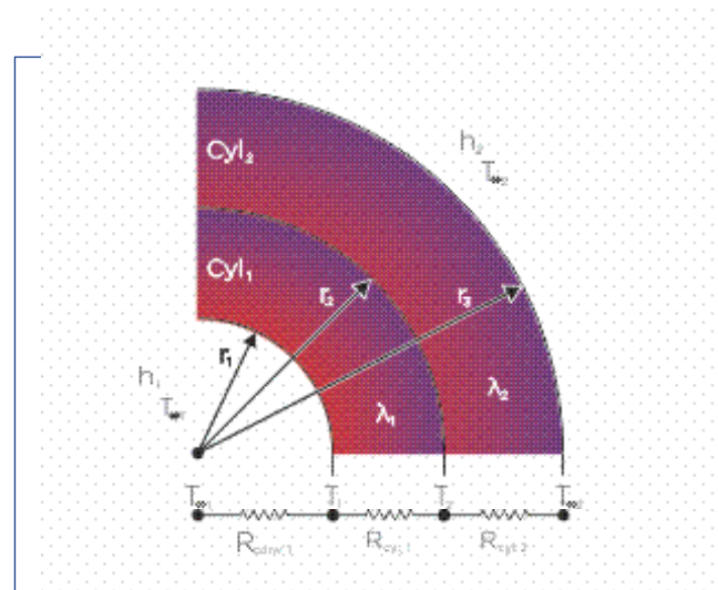
Figure 19. Network of thermal resistors for transferring heat through a cylinder of two layers exposed
