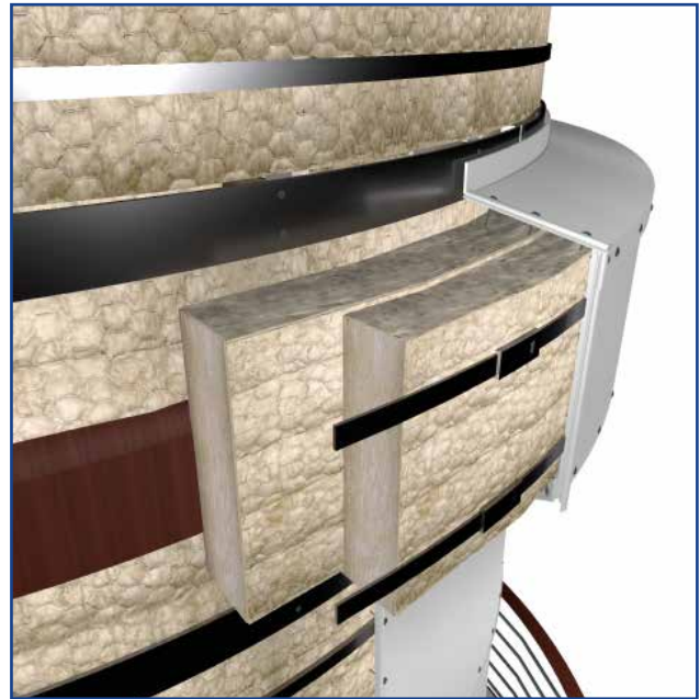
Figure 19. COLUMN DETAIL 1
