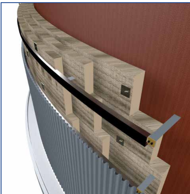
Figure 22. STORAGE TANK DETAIL 1 (Wired Mats)
