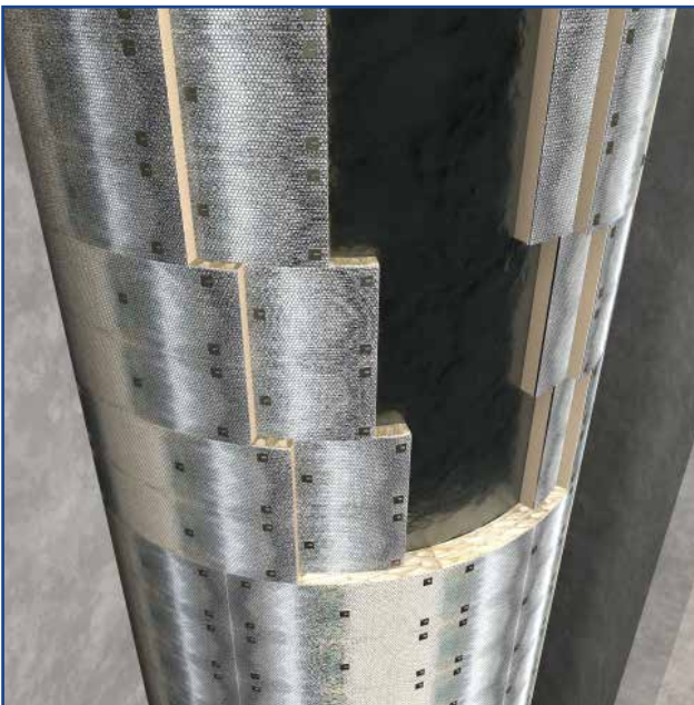
FIGURE 33. EXHAUST STACK DETAIL 1
