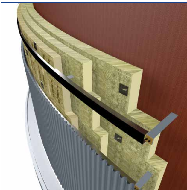
Figure 25. STORAGE TANK DETAIL 1 (Panels)
