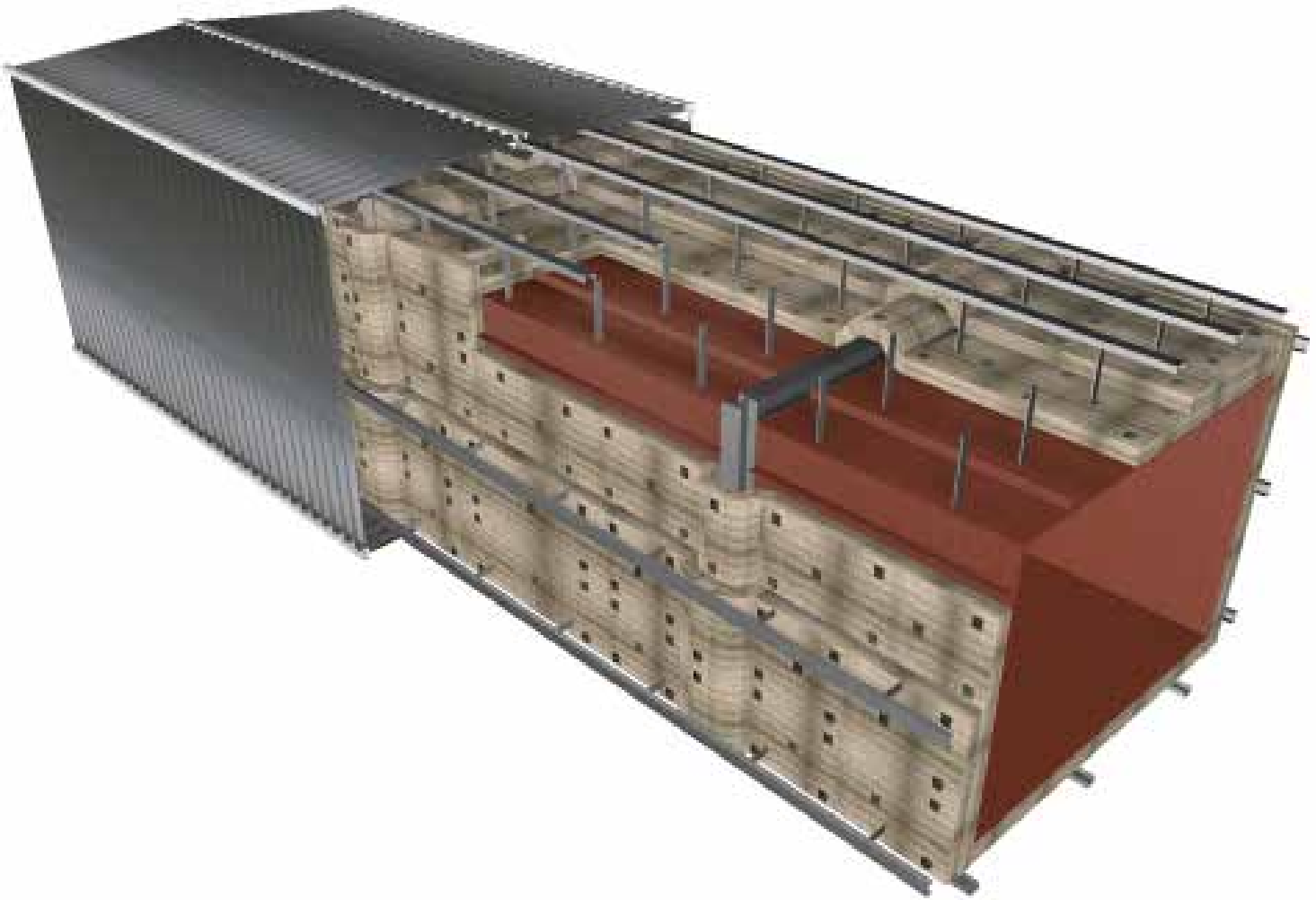
Figure 29. EXHAUST DUCT
